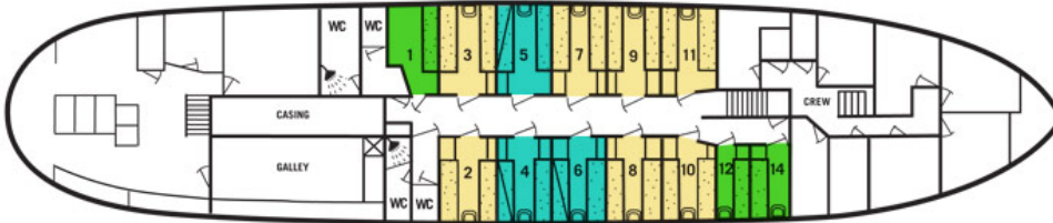
MAIN DECK
