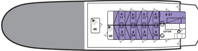
SHELTER DECK
